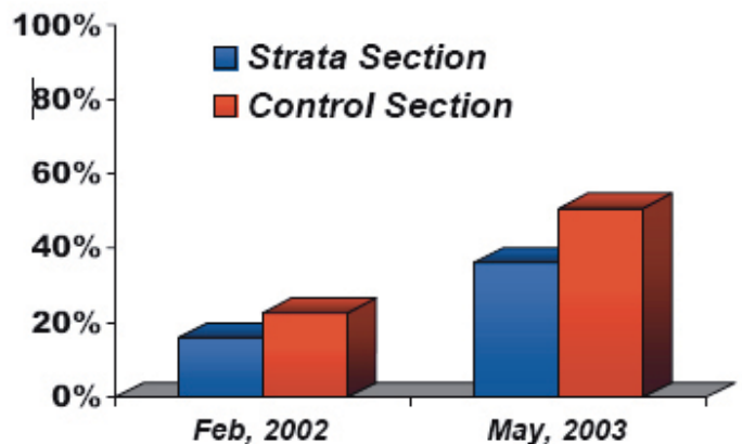
Percent Reflective Cracking Performance 2 years after construction.
